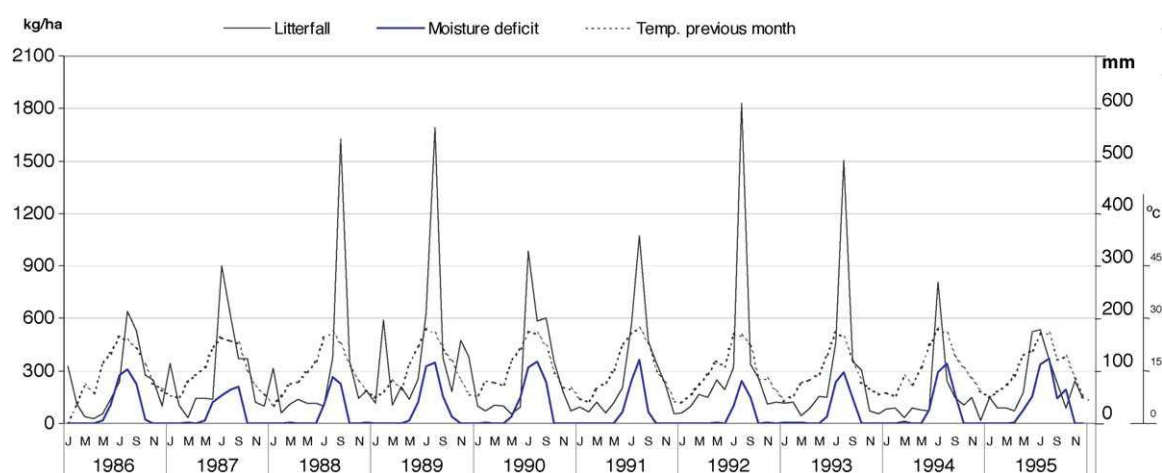
Fig. 4. Evolution of monthly litter fall ( \text{kg ha}^{-1} of dry matter, mean of all treatments), mean monthly temperature ( ^{\circ}\text{C} ) and moisture deficit (mm) during the period of time studied.
