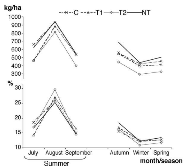
Fig. 3. Absolute ( \text{Kg ha}^{-1} of dry matter) and relative (%) mean values of litter fall per treatment and seasons of the year (relative values in relation to total annual litter fall). Summer has been divided into the 3 months considered.
