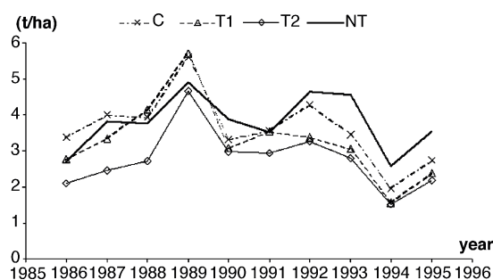
Fig. 2. Evolution of total annual litter fall along the decade of study per treatments. C: control; T 1 : moderate thinning regime; T 2 : heavy thinning regime; NT: never thinned.
