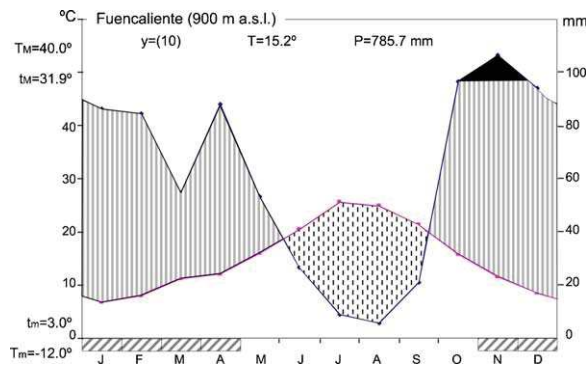
Fig. 1. Climatic diagram (Walter, 1963) of the experimental site during the studied period of time. y : number of years considered; T : mean annual temperature ( ^{\circ}\text{C} ); P : mean annual amount of precipitation (mm); T_M : absolute maximum temperature ( ^{\circ}\text{C} ); t_M : mean daily maximum temperature of the hottest month ( ^{\circ}\text{C} ); t_m : mean daily minimum temperature of the coldest month ( ^{\circ}\text{C} ); T_m : absolute minimum temperature ( ^{\circ}\text{C} ). Obliquely striped area shows months with an absolute minimum below 0^{\circ}\text{C} .
