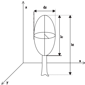
Figure 1. Single tree variables use to characterize the canopy stratum; ht : total height, dc : crown diameter and lc : crown length. To estimate the relative abundance of foliage in each stratum for the FHD calculation, the crown of the trees was considered as an ellipsoid of revolution with z axis as revolution axis.
