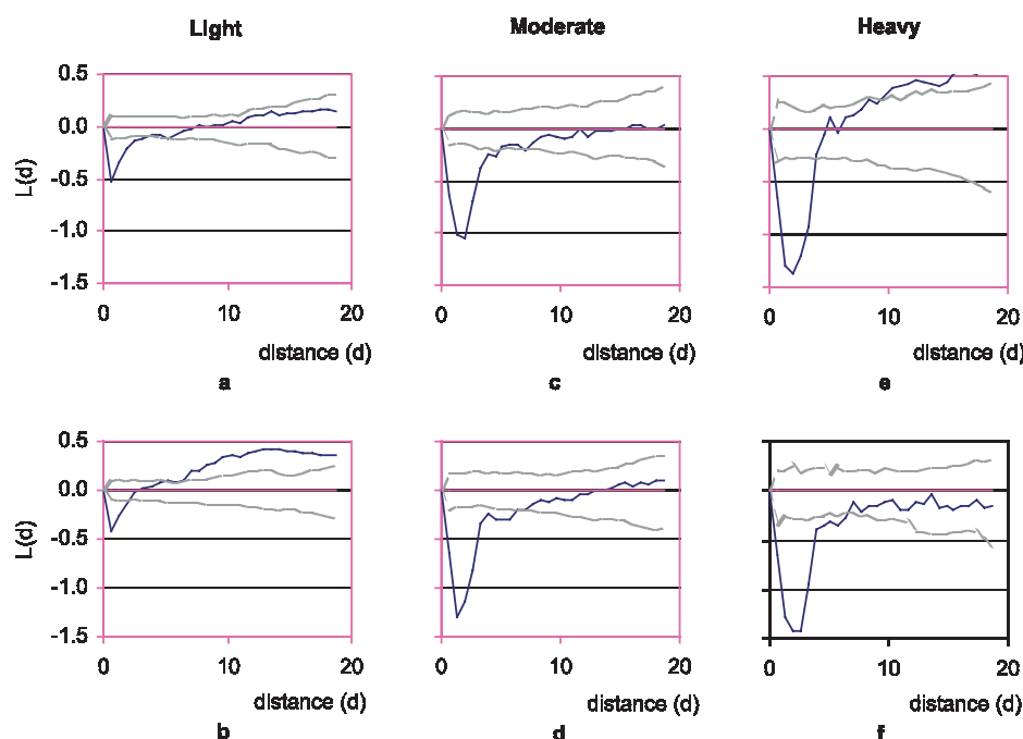
Figure 3. Analysis of the spatial pattern of trees in Q. faginea plots (a and b: light thinning; c and d: moderate thinning; e and f: heavy thinning; 2 plots for each treatment) using the transformation L(d) of Ripley's function K(d) . Solid lines: K function value for the real distribution of the trees; grey lines: 90% confidence interval boundaries of L(d) of a Poisson distribution.
