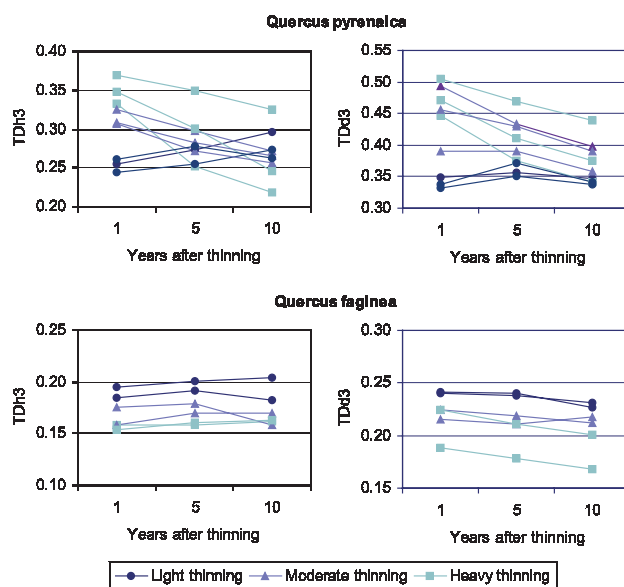
Figure 5. Evolution of Gadow's differentiation index calculated using three neighbours for height ( TDh3 ) and diameter ( TDd3 ) in Q. pyrenaica plots (above) and in Q. faginea plots (below). Different plots have been represented by different lines to show same treatment variability.
