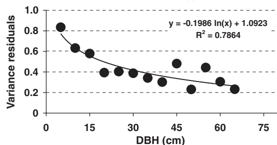
Fig. 7. Estimation residuals (predicted-observed) versus predicted DBH as an illustration of potential heteroskedasticity for age independent formulations. Residual variance by diameter class and estimated variance function (i.e., weigh, w_i ) applied in T2 and T5s.
