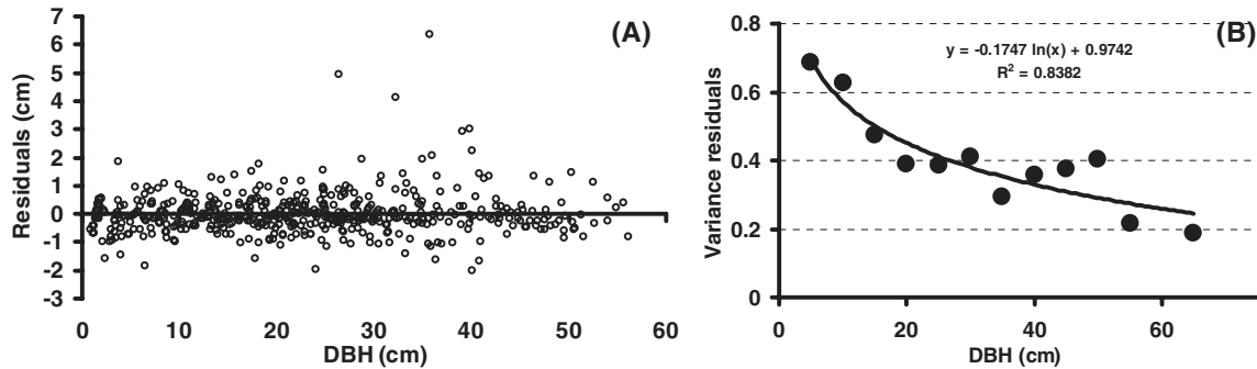
Fig. 2. Estimation residuals (predicted–observed) versus predicted DBH as an illustration of potential heterokedasticity for the E5 growth model: (A) E5 for the 25 series and (B) E5 2 for the 115 series, variance for each diameter class and estimated variance function (i.e., weight, w_i ) applied.
