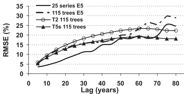
Fig. 6. Relative root mean square error (RMSE) by lag of prediction for E5 (solid line), E5 2 (broken line), T2 (circles) and T5s (triangles).
