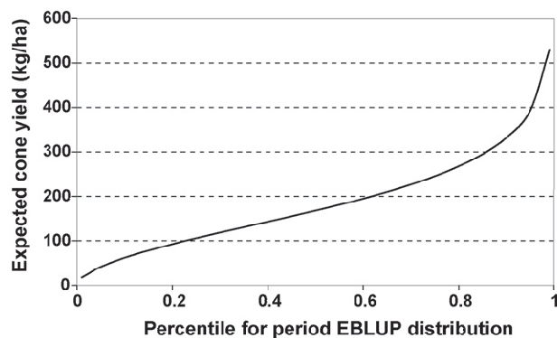
Fig. 6. Expected cone yield (kg/ha) in validation plot no. 26 as a function of the percentile of the distribution for random period effects (mean zero, variance 0.1142).
