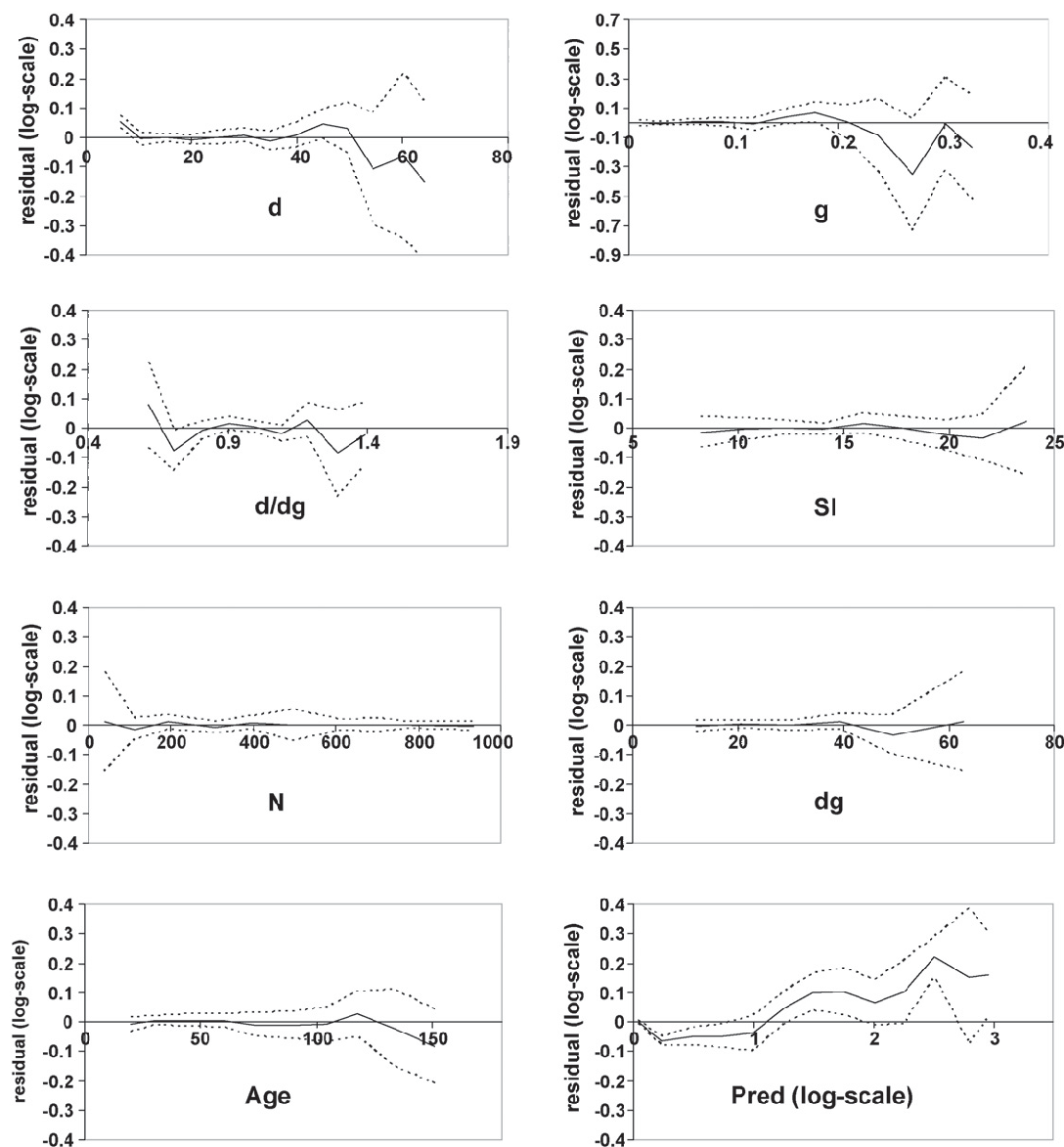
Fig. 4. Mean conditional residual in log-scale (solid line) as a function of predicted value and explanatory stand and tree level covariates. Dotted lines indicate standard error for the mean.
