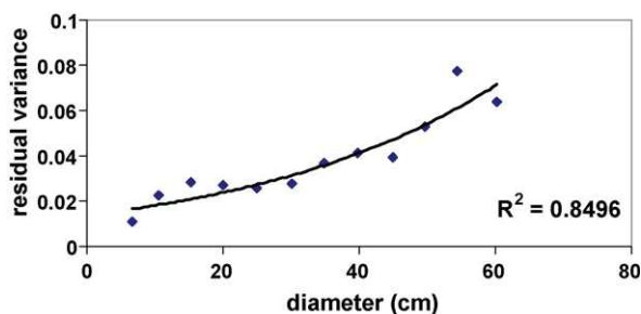
Fig. 2. Residual variance for basic model (dots) and fitted variance function (solid line).
