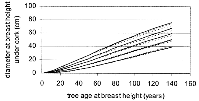
Figure 8. Diameter growth curves obtained using the Richards (RCn) function, both without differentiating the two regions (continuous line) and with differentiation: Catalonia (dashed line) and the Natural Park of "Los Alcornocales" (dotted line). (The diameter growth curves were represented in terms of each site quality class and mean values of height to diameter ratio for each site quality class.)
