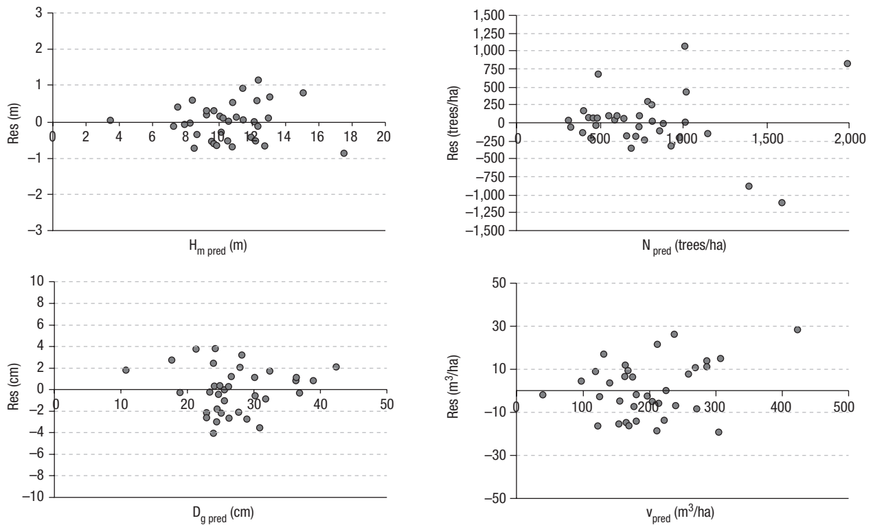
Figure 3. Residuals versus predicted values ( H_{m\text{ pred}} , N_{\text{pred}} , D_{g\text{ p-reg}} , V_{\text{pred}} ) for HD models.
